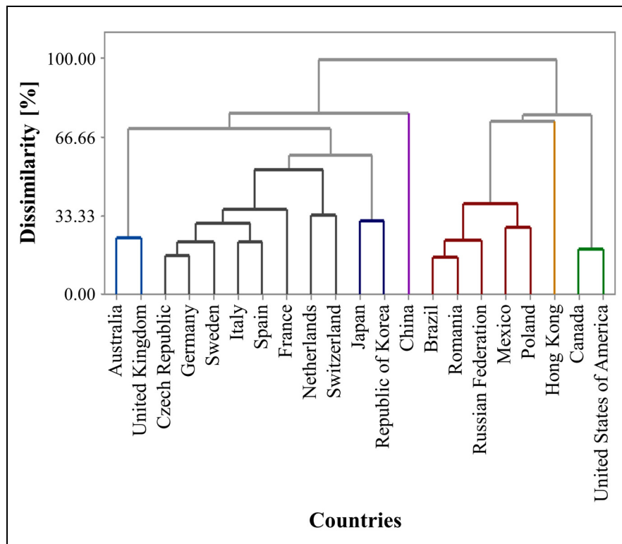
Figure 4. Dendrogram of the Euclidean distance between countries considering the composition of service portfolio.
